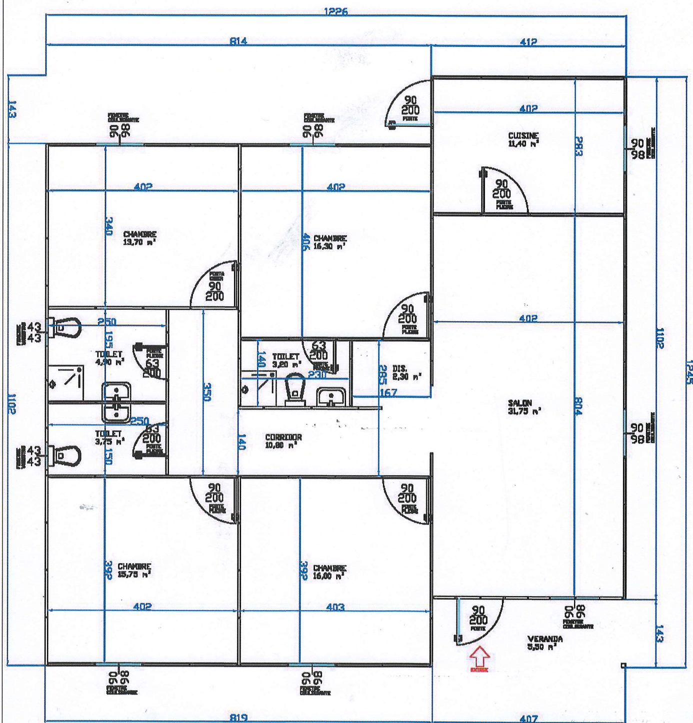
MOD. D - 'F5' - 141,00 m 2 - PLAN TECHNIQUE
